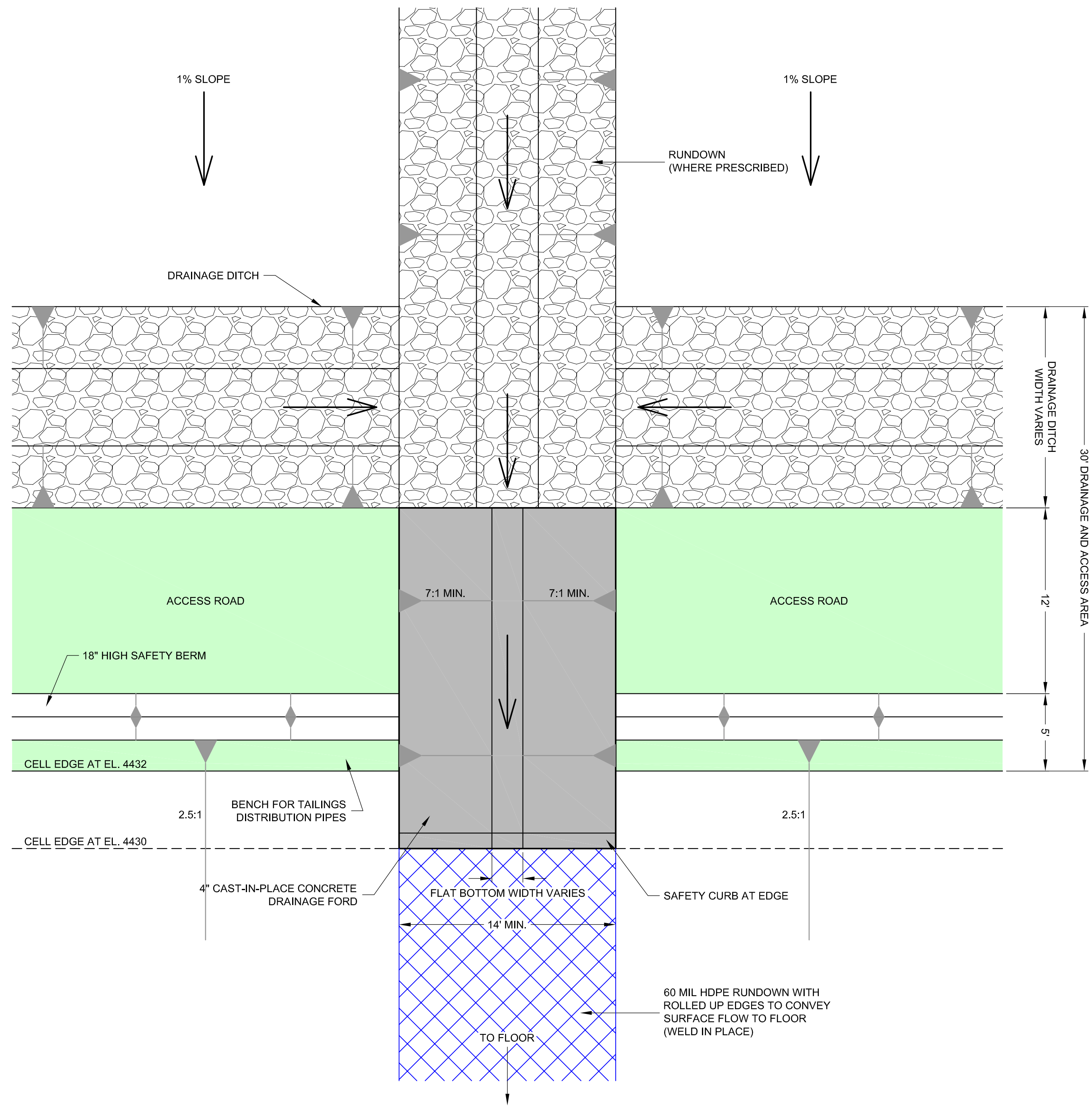
TYPICAL PLAN VIEW DRAINAGE FORD SCALE: 1" = 5'
